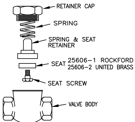
HORIZONTAL SPRING LOAD CHECK VALVE 25606
