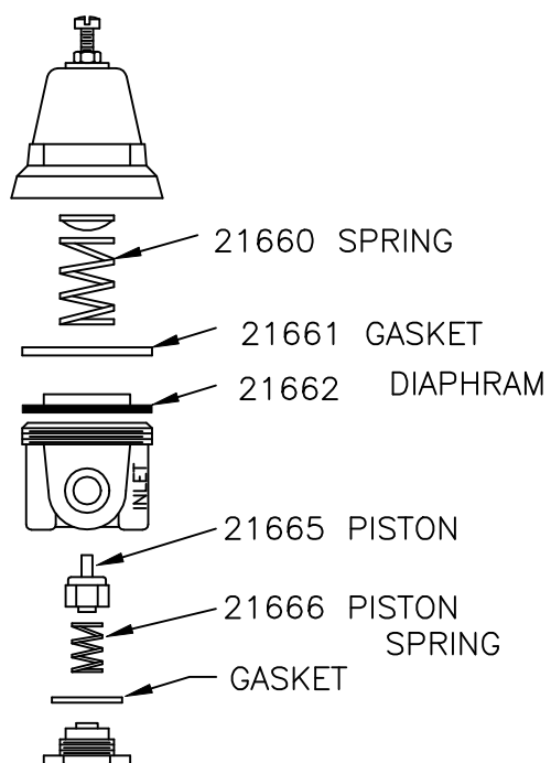
1/4" REGULATOR 16048
